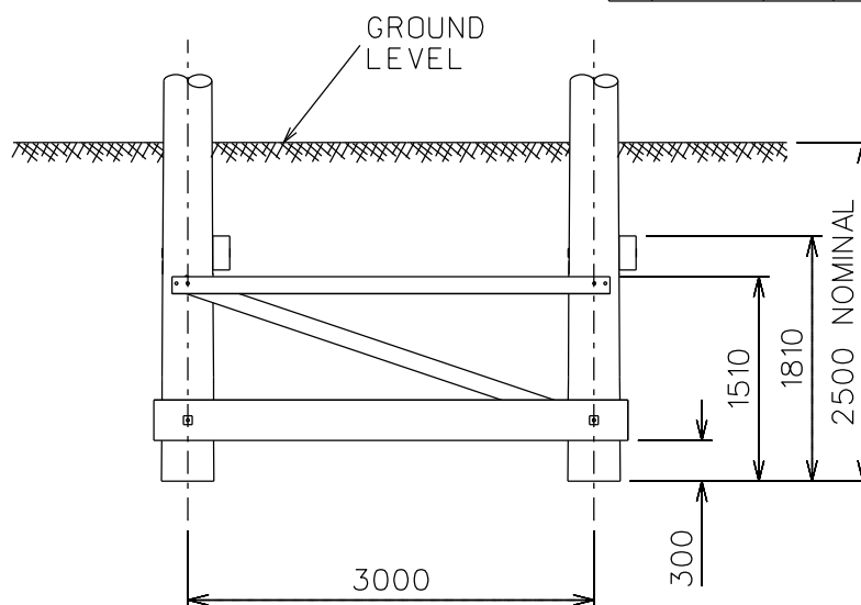
15m POLE FRONT ELEVATION
